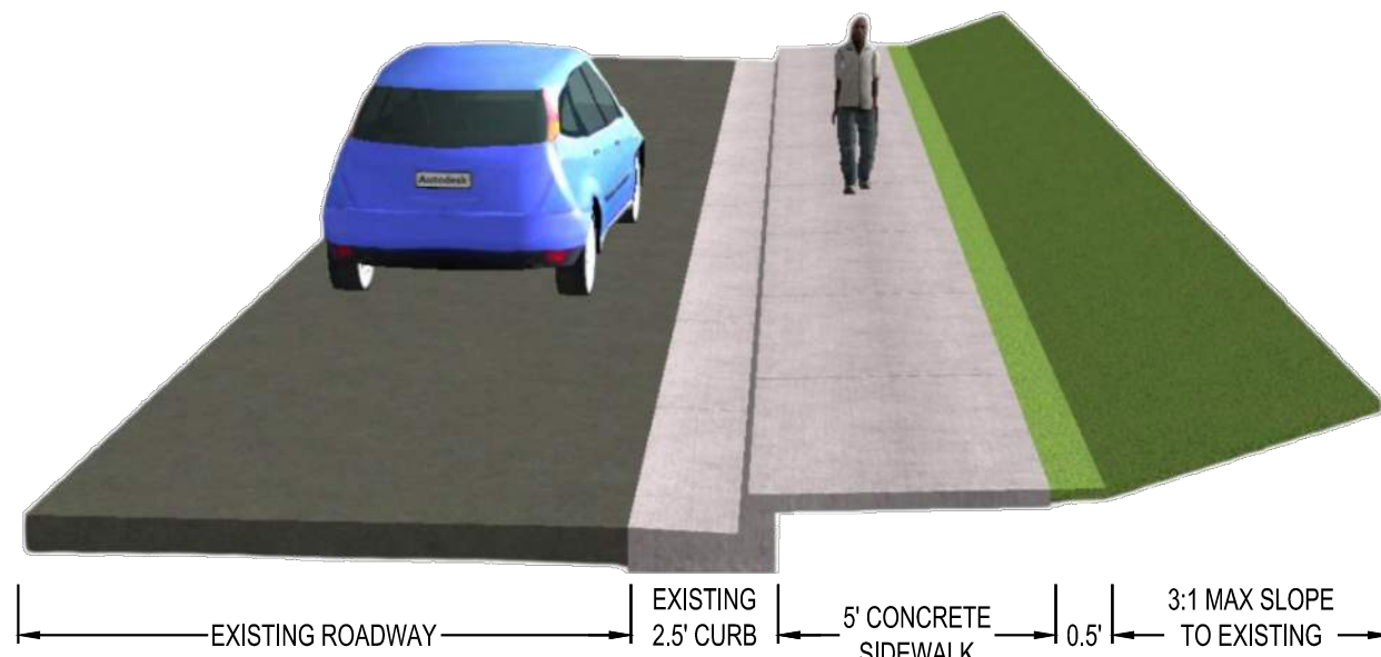
TYPICAL SECTION NO. 1
