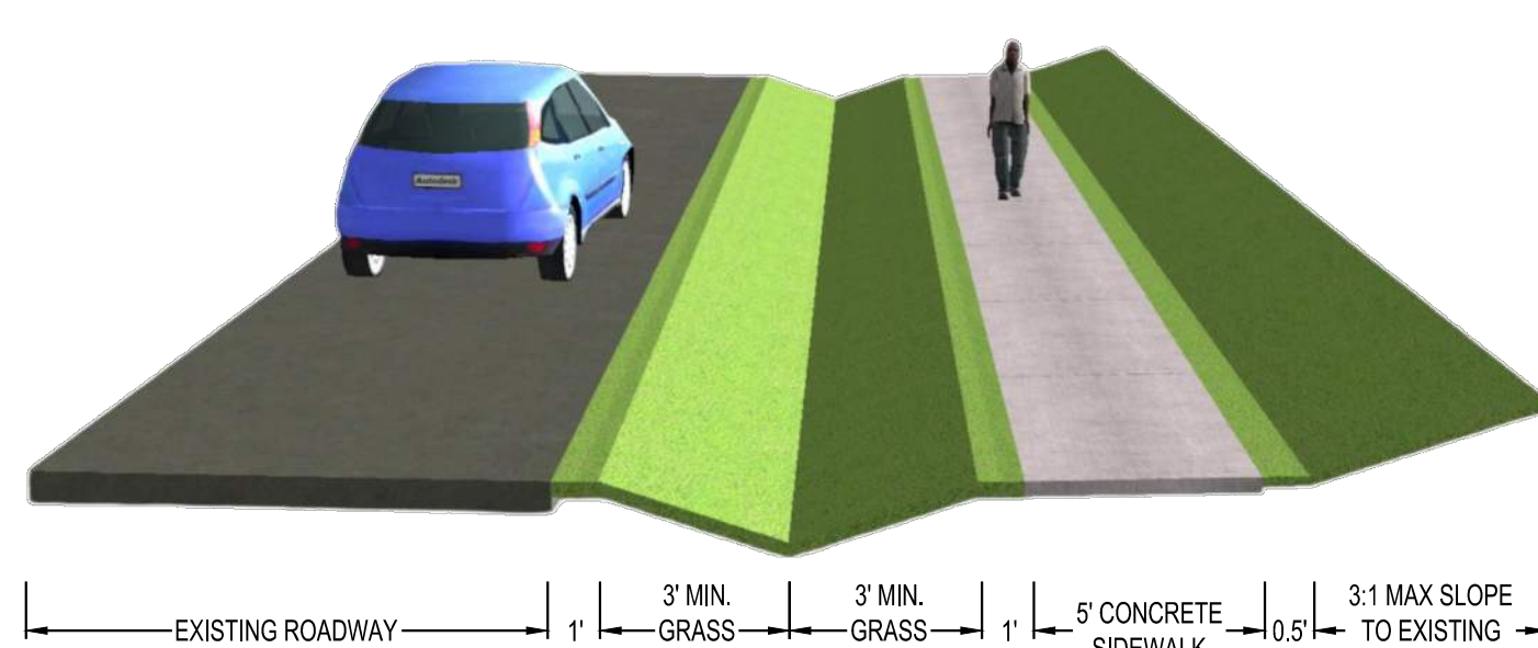
TYPICAL SECTION NO. 3
